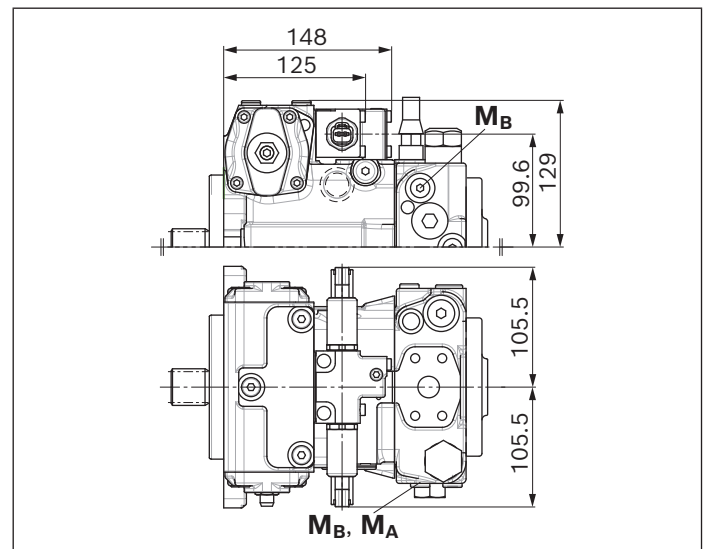
▼ ET – Electric control, direct operated, two FTDRE
