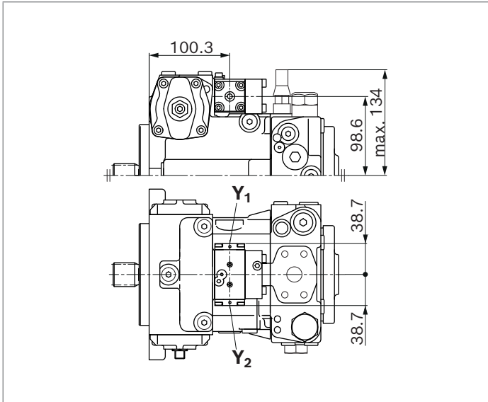
▼ EP – Proportional control, electric
