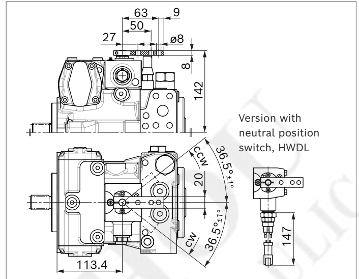
▼ HW – Proportional control, hydraulic, mechanical servo
