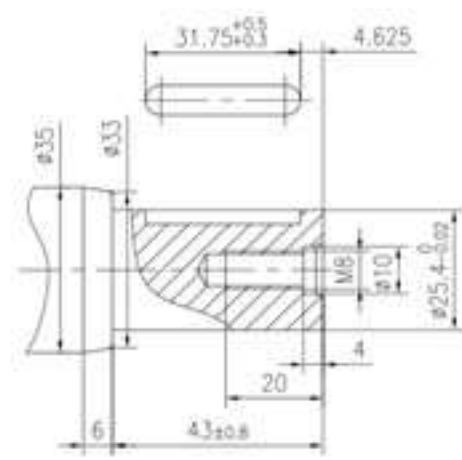
Output Shaft
