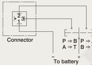
Electric wiring example
